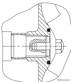
Impeller screw
